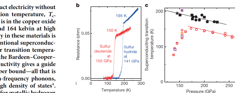
Figure 2 | Pressure and temperature effects on T_c of sulfur hydride and sulfur deuteride. a , Changes of resistance and T_c of sulfur hydride with
