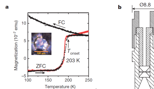
Figure 4 | Magnetization measurements. a , Temperature dependence of the magnetization of sulfur hydride at a pressure of 155 GPa in zero-field cooled (ZFC) and 20 Oe field cooled (FC) modes (black circles). The onset temperature is T_{\text{onset}} = 203(1) K. For comparison, the superconducting step obtained for sulfur hydride from electrical measurements at 145 GPa is shown by red circles. Resistivity data ( T_{\text{onset}} = 195 K) were scaled and moved
